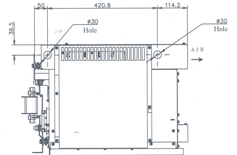
<RIGHT VIEW>
